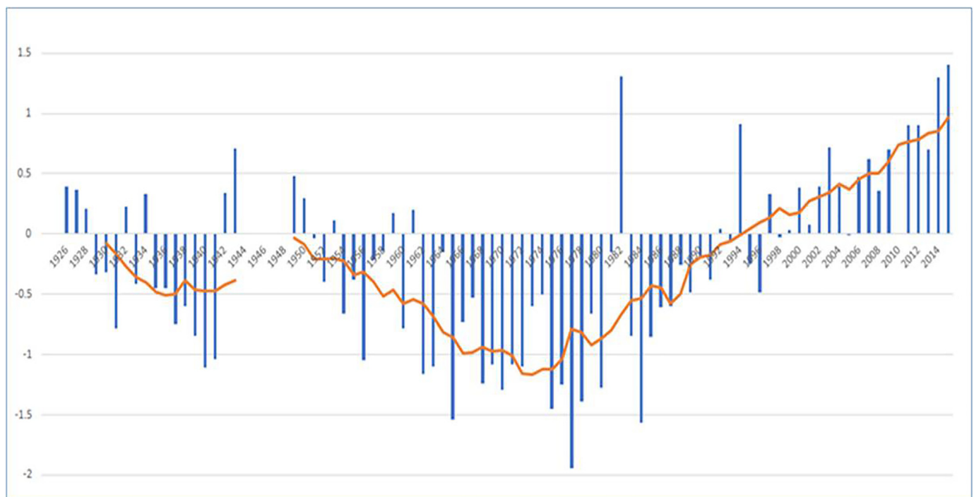
Fig. 3. Bolzano, Italy: trend of annual temperatures based on differences from mean value (°C) for the 1926–2015 period.
